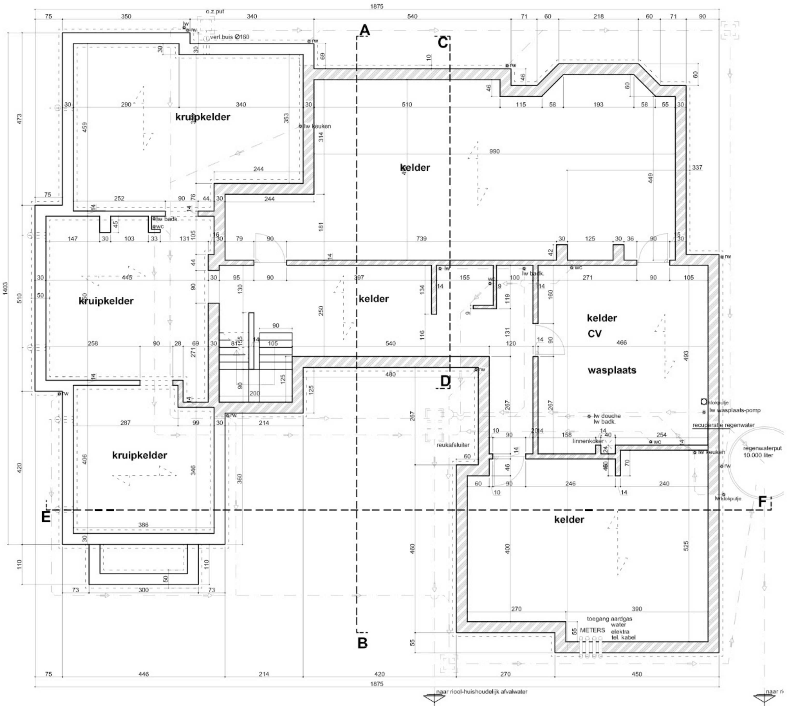
KELDER_FUNDERING_RIOLERING
